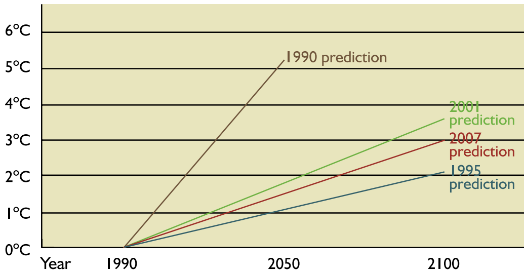
Predicted Temperature Increases
