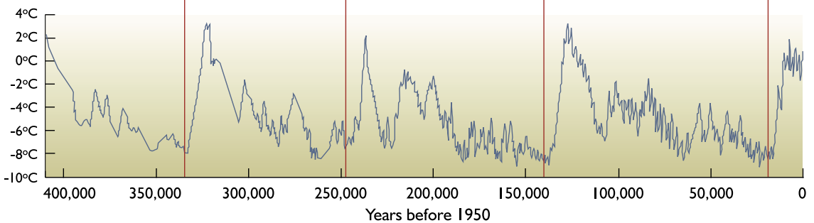
Temperature Difference from 1950
